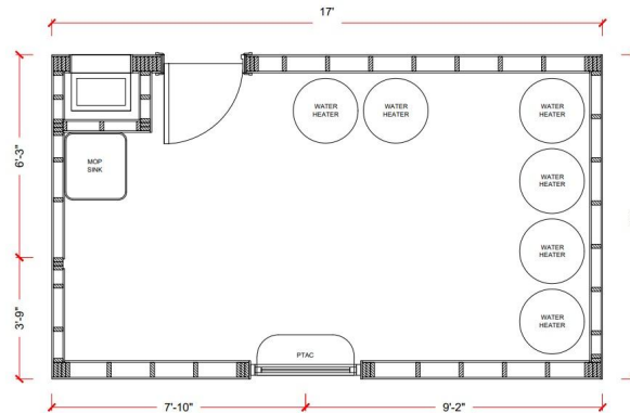
LAUNDRY UNIT SCALE 1" : 2'
