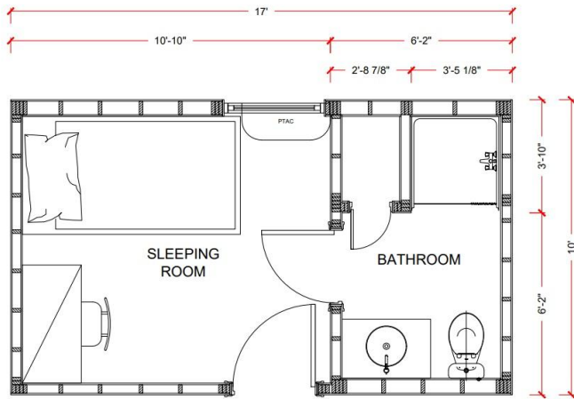
A1 SLEEPING UNIT SCALE 1" : 2'
