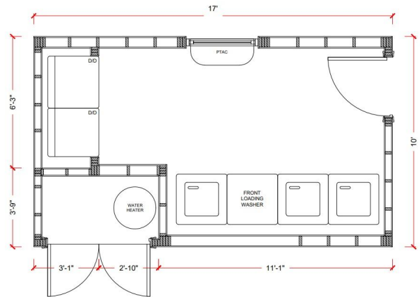
LAUNDRY UNIT SCALE 1" : 2'
